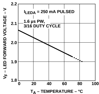
Figure 3. LED Forward Voltage vs. Temperature.
