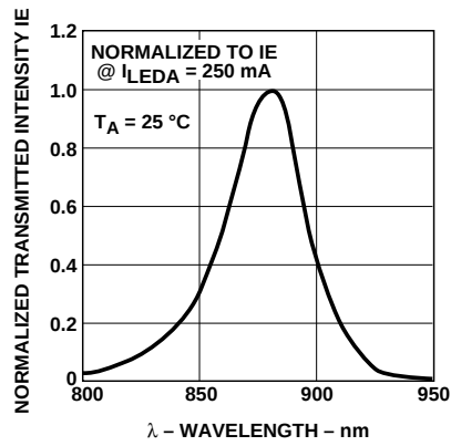
Figure 6. Transmitted Intensity vs. Wavelength.
